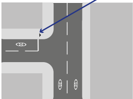
Typical side road detail
